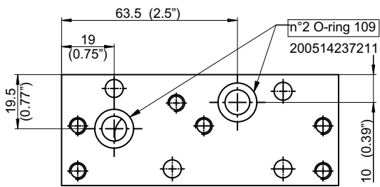
Housing side
