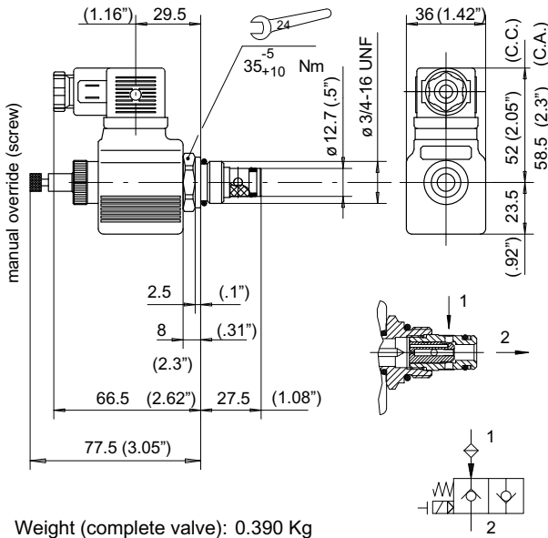
Weight (complete valve): 0.390 Kg
