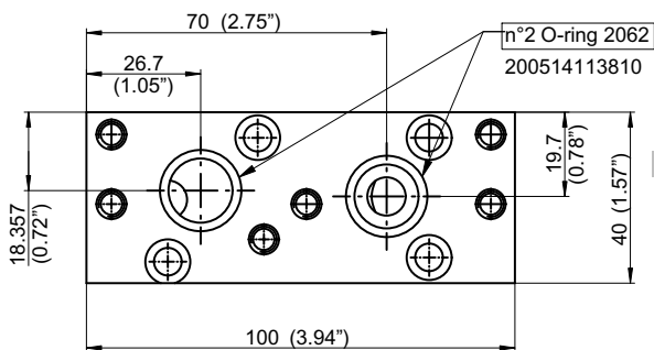
Block side
