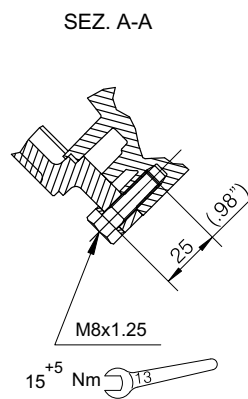
Fixing system
