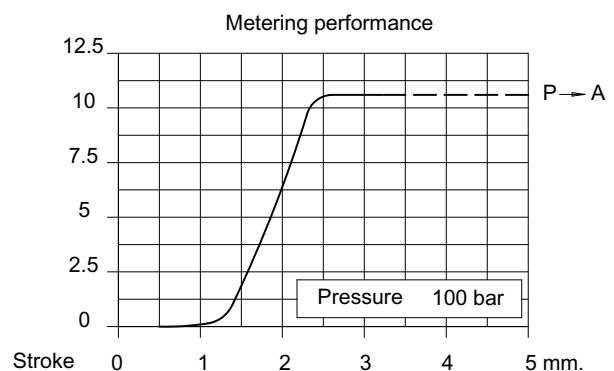
Performances (Viscosity 37 mm 2 /s at 40° C)
