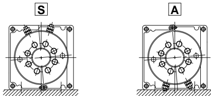
Motor mounting position Standard positions
