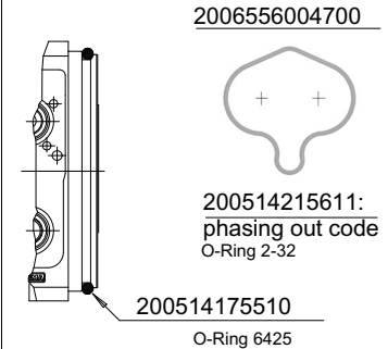
O-Rings kit 200974200400
