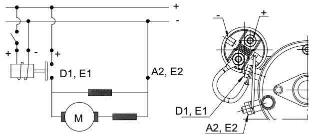
Electric diagram
