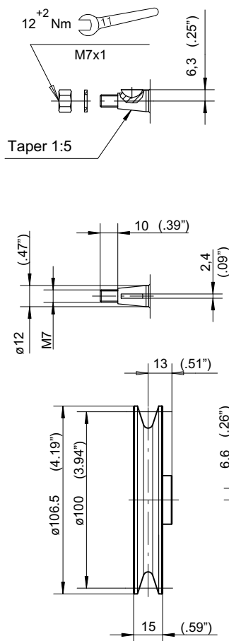
Shaft end
