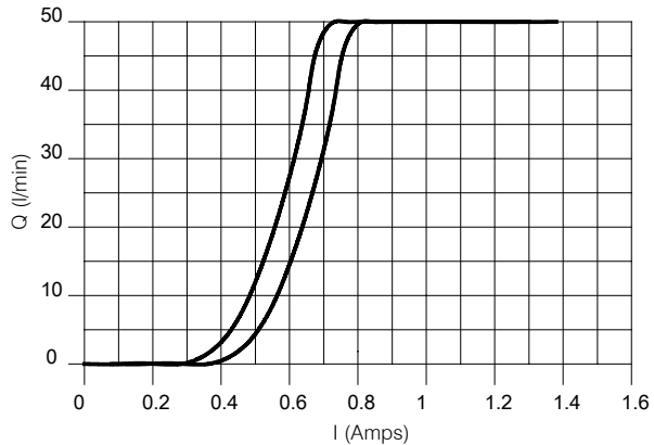
Typical hysteresis
