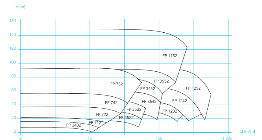
Characteristic curves of the Fristam series FP (transportation of water); n = 2,900 \text{ min}^{-1}
