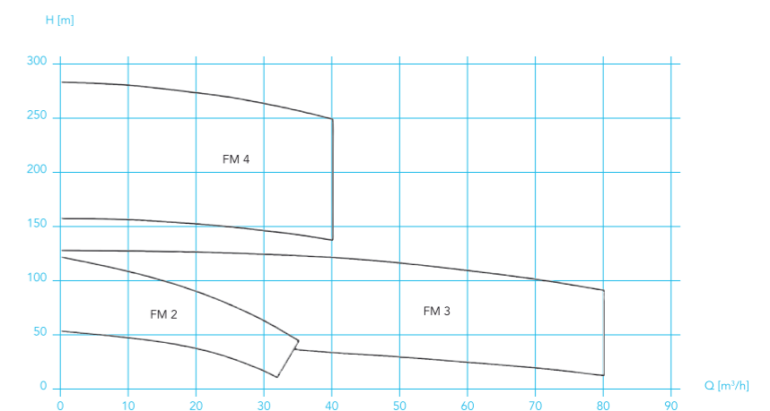
Characteristic curves of the Fristam series FM (transportation of water); n = 2,900 \text{ min}^{-1}
