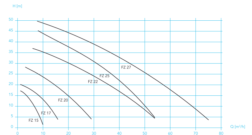
Characteristic curves of the Fristam series FZ (transportation of water); n = 1,450 \text{ min}^{-1}
