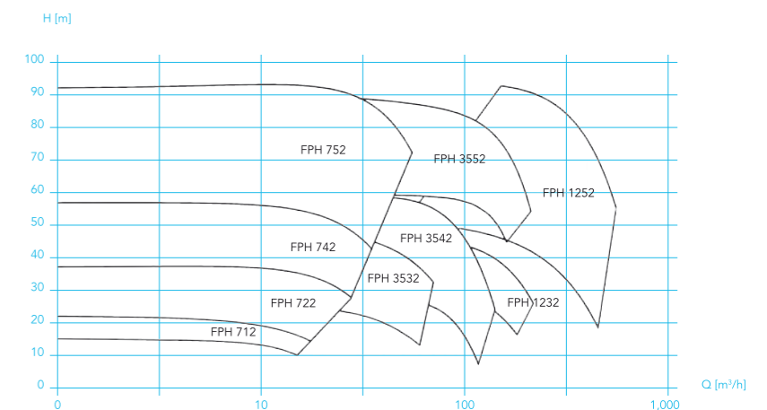
Characteristic curves of the Fristam series FPH (transportation of water); n = 2,900 \text{ min}^{-1}
