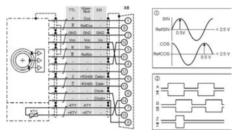
Encoder connection
