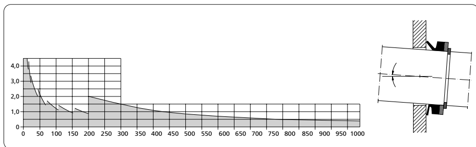
Diagram 11. Maximum permissible misalignment for V-rings of the VR1 and VR2 designs
