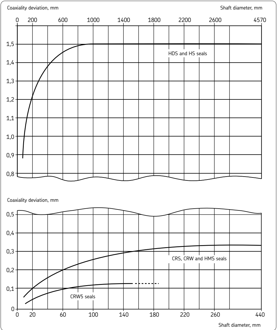
Diagram 6. Maximum permissible deviation from coaxiality as a function of shaft diameter
